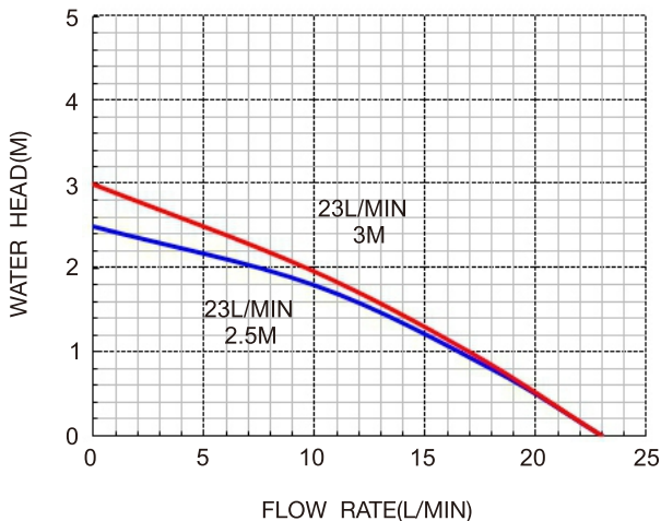
TA50 Performance
